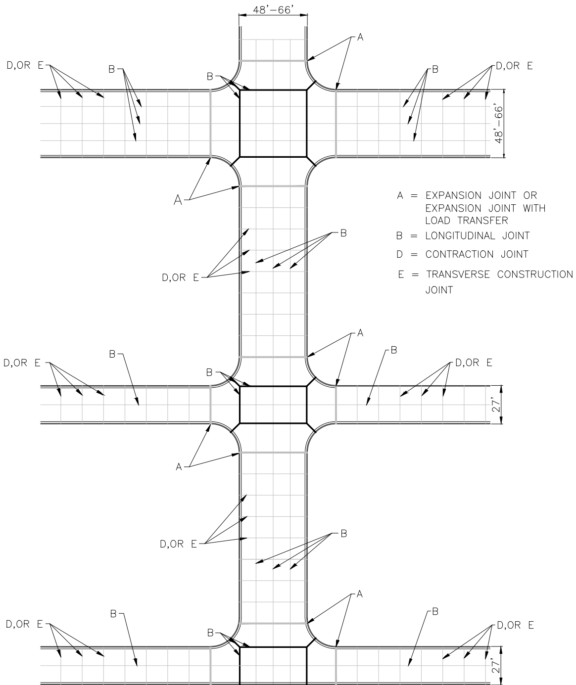
TYPICAL STREET JOINT DETAIL
