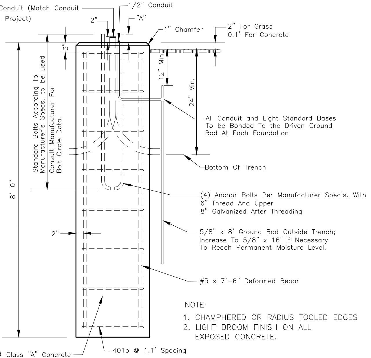
DETAIL OF LIGHT STANDARD FOUNDATION
