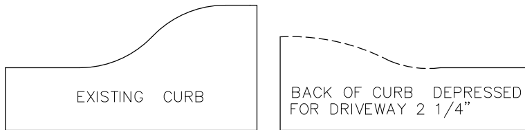
CONCRETE CURB TYPE I-B
