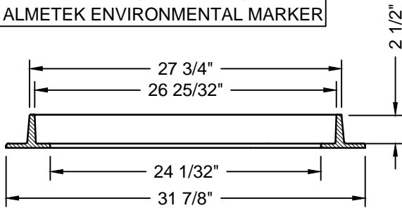
FRAME SECTION B-B
