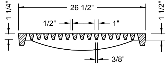
GRATE SECTION B-B
