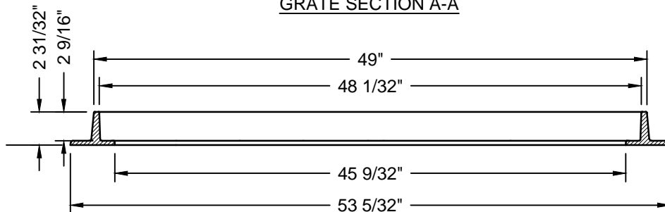
FRAME SECTION A-A
