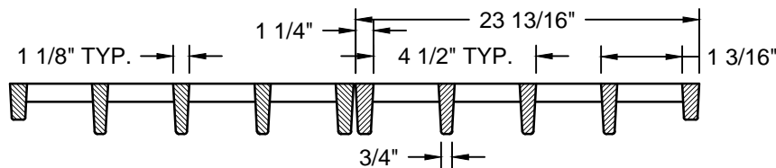
GRATE SECTION A-A
