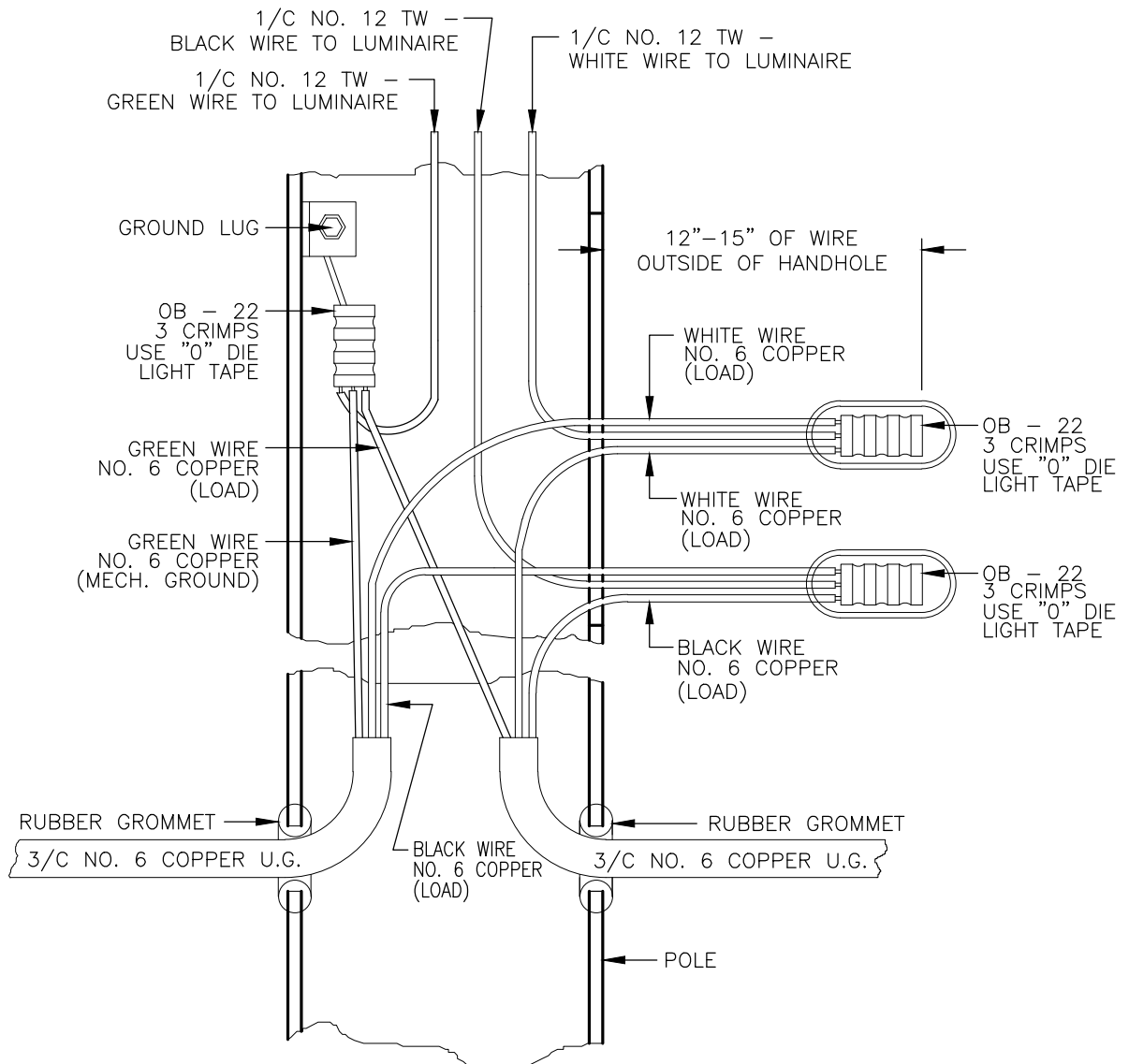
TYPICAL 120 VOLT UNDERGROUND INSTALLATION
