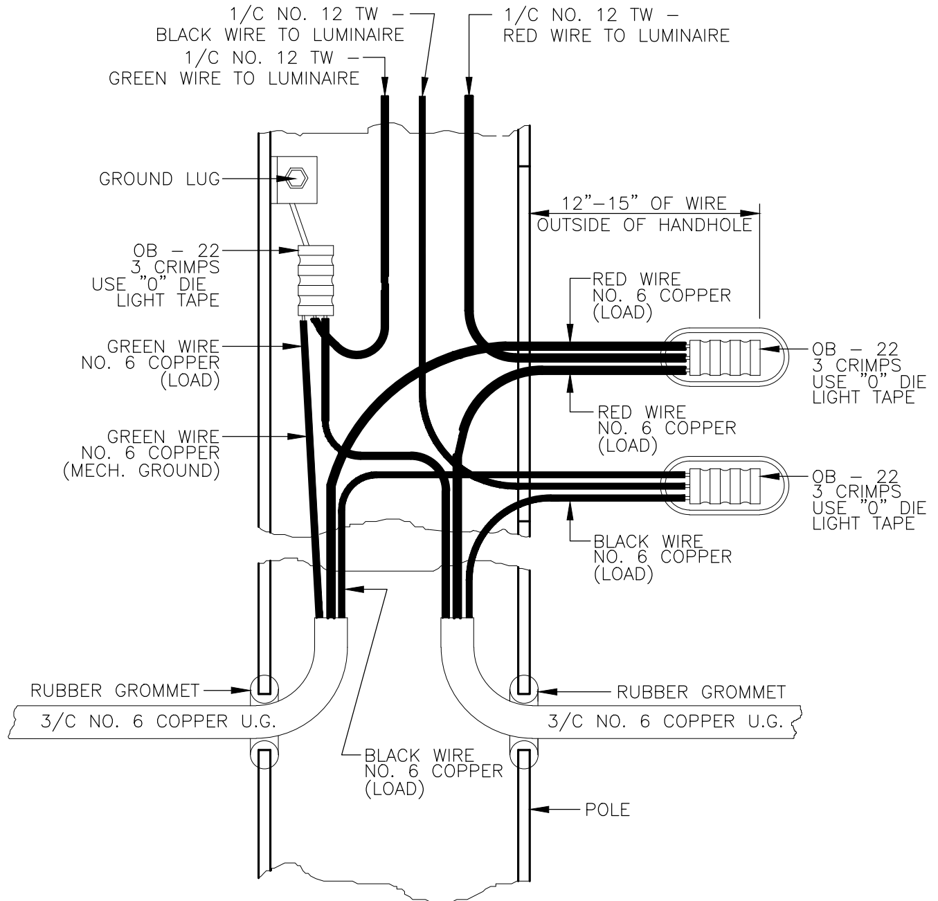
TYPICAL 240 VOLT UNDERGROUND INSTALLATION
